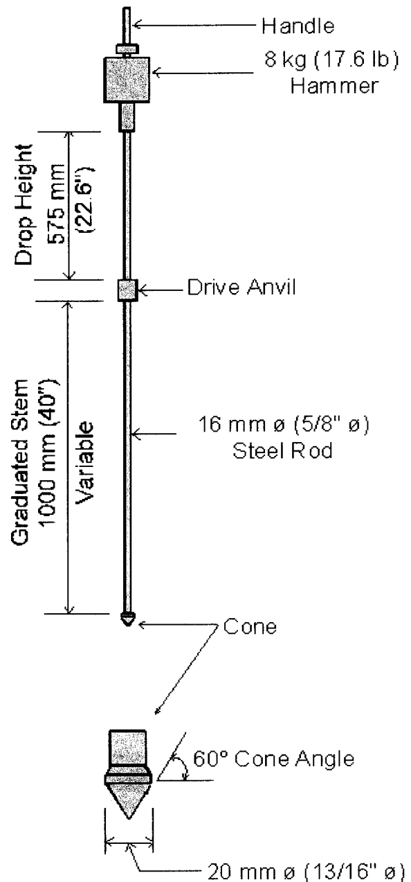
Figure 1: Schematic of DCP
