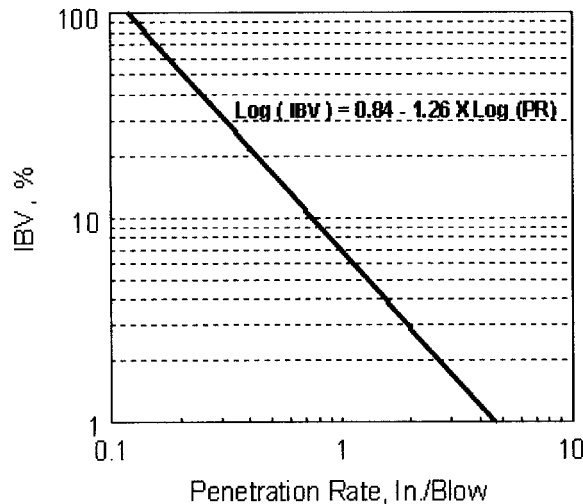
Figure 2: IBV - PR Correlation
