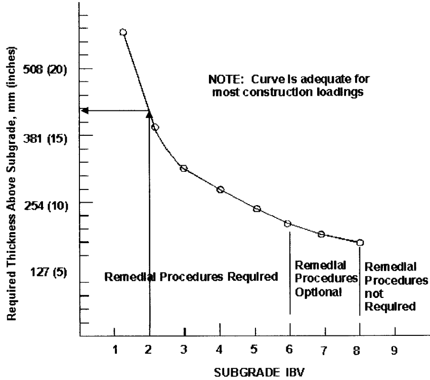
Figure 3: IBV-Based Thickness Design for Granular Backfill and Subgrade Modification
